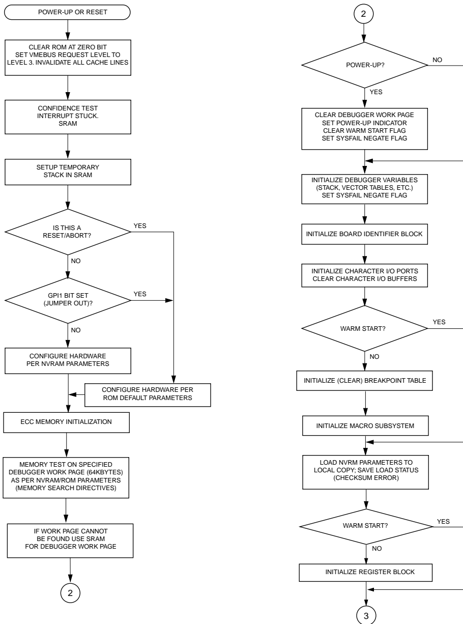
Figure 1-1. 172Bug Start-up Flow (Sheet 1 of 3)
