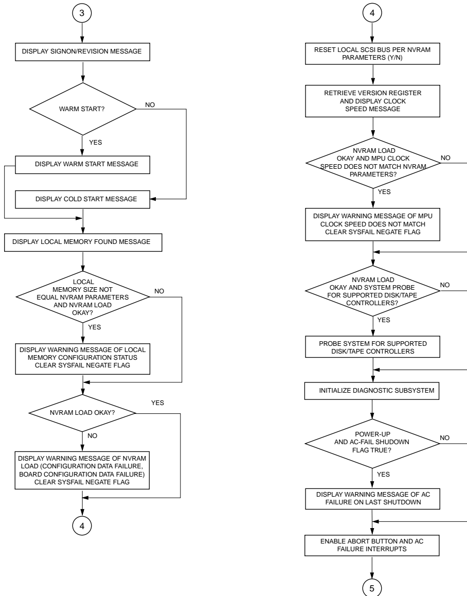
Figure 1-1. 172Bug Start-up Flow (Sheet 2 of 3)
