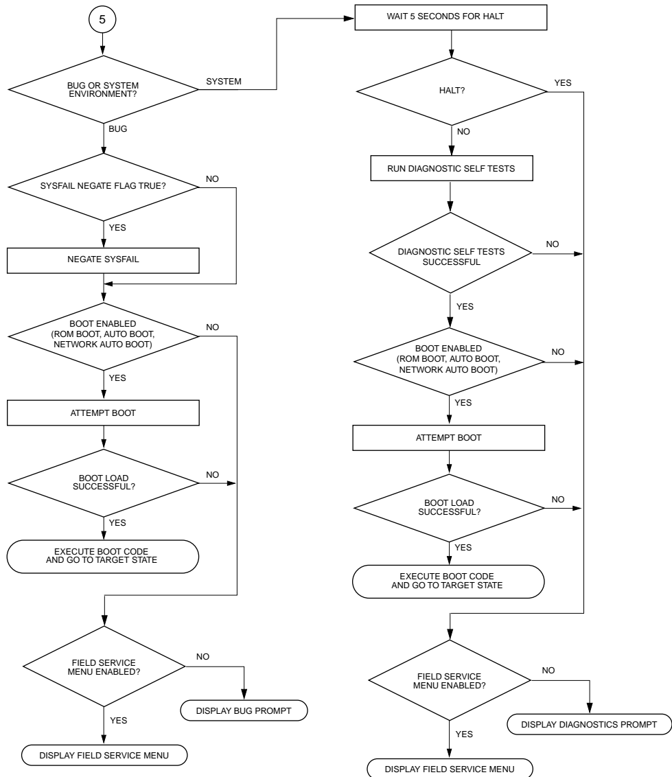
Figure 1-1. 172Bug Start-up Flow (Sheet 3 of 3)
