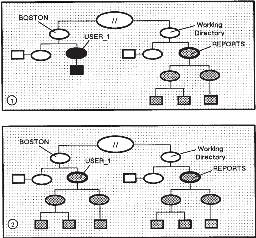
Figure 7-7. Replacing a Directory Tree
