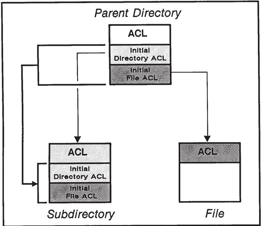
Figure 8-4. Initial ACLs for Files and Directories
