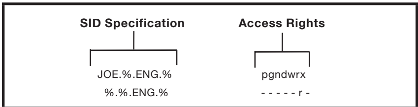
Figure 8-2. Sample ACL Entries
