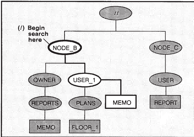
Figure 1-4. A Sample Path Beginning at the Node Entry Directory
