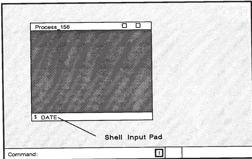
Figure 6-1. The Shell Process
