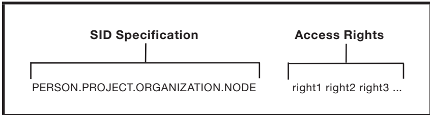
Figure 8-1. Structure of an ACL Entry
