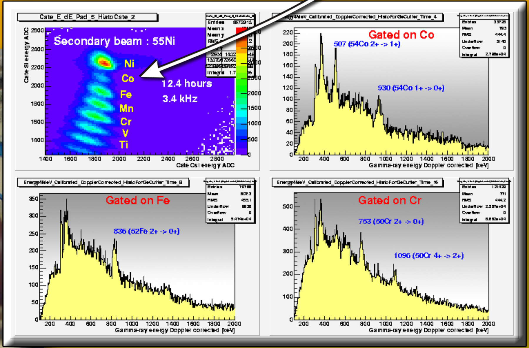
Fragmentation products
