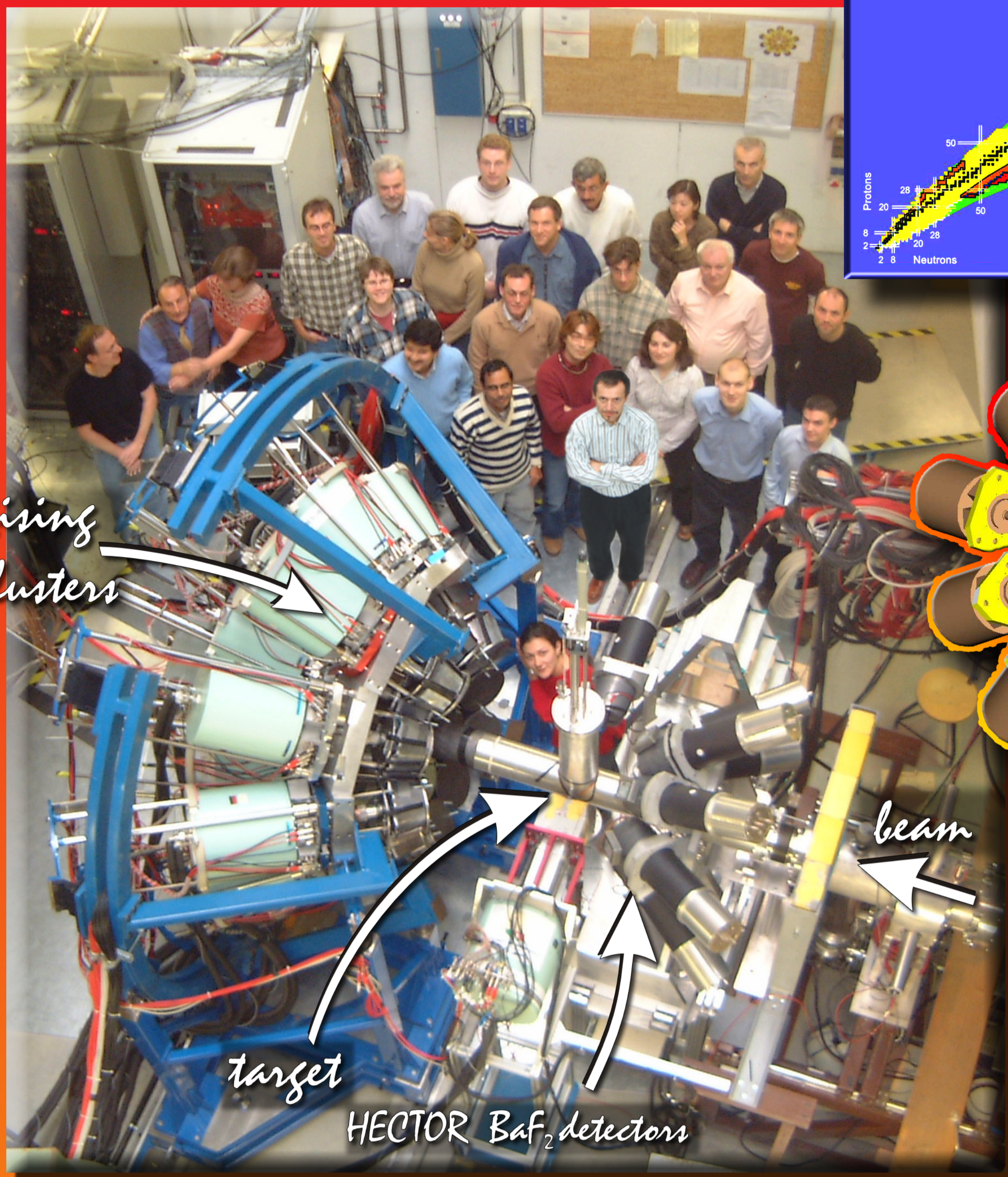
Last phase of mounting the clusters
