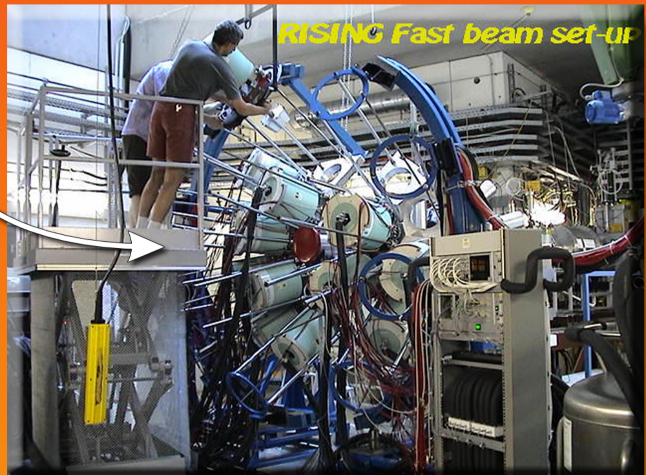
Last phase of mounting the clusters
